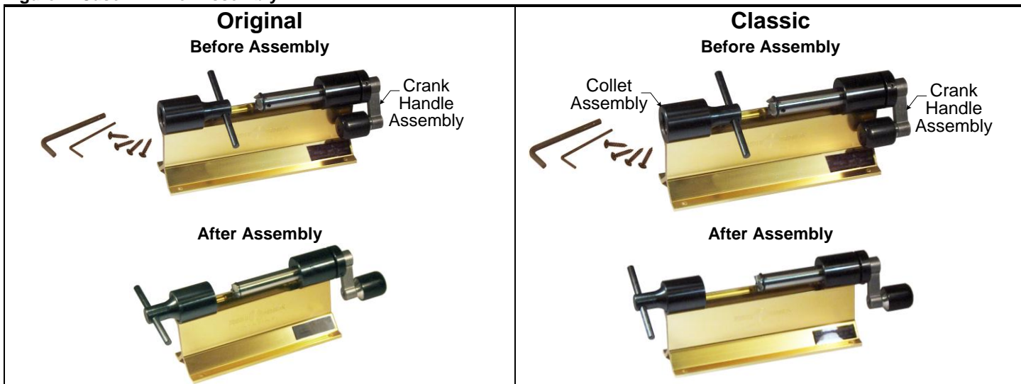
Figure 1. Case Trimmer Assembly
